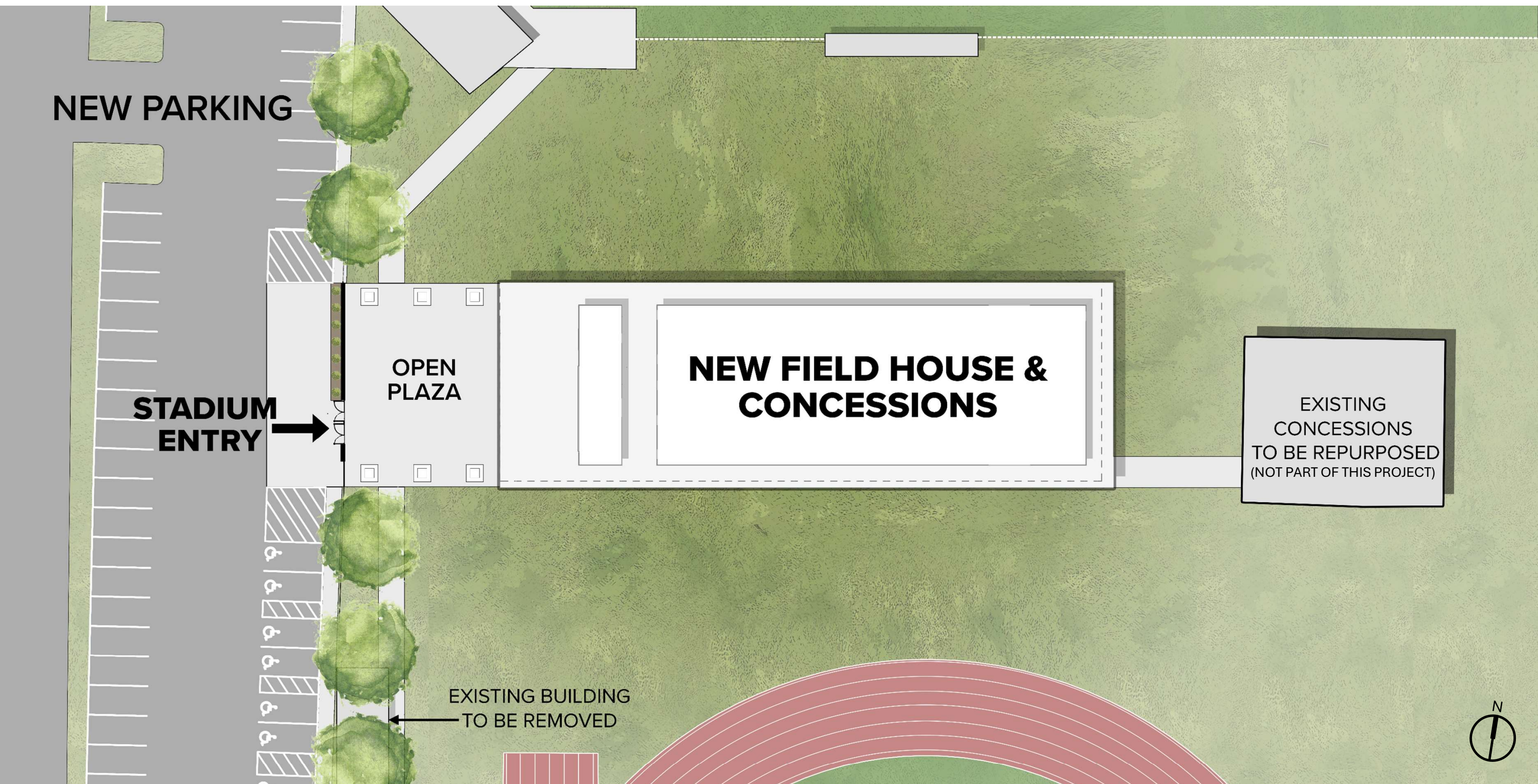
FIELDHOUSE - SITE PLAN
